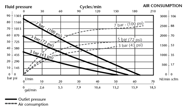
SAE 10, 21 °C ( 70 °F) CAPACITY CURVE
