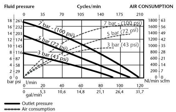
SAE 10, 21 °C ( 70 °F) CAPACITY CURVE
