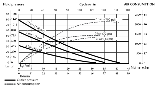
NLGI-2, 21 °C (70 °F) CAPACITY CURVE
