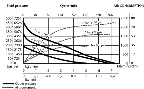
NLGI-2, 21 °C (70 °F) CAPACITY CURVE
