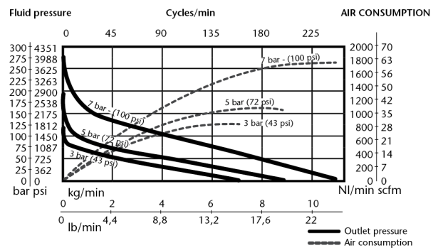
NLGI-2, 21 °C (70 °F) CAPACITY CURVE
