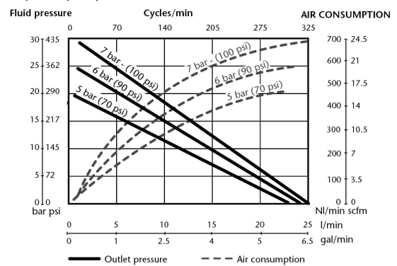
SAE 30, 23 °C (73 °F) CAPACITY CURVE
